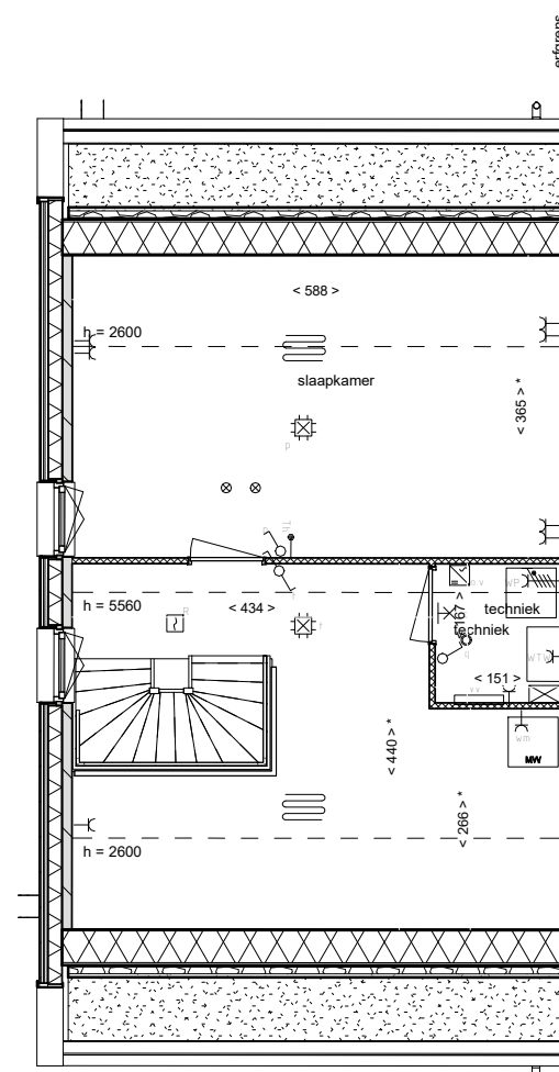
zolder
